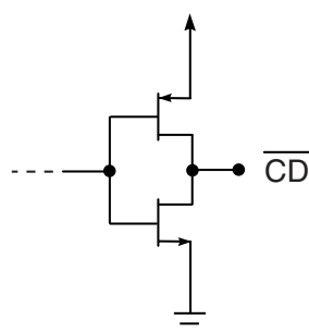
Figure 3-5: \overline{CD} Circuit
